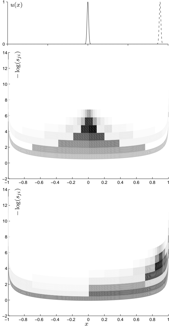
Figure 4: Coefficient scalogram of the transform of a Gaussian bump with center x_c = 0 (center) and x_c = 0.9 (bottom). In both cases, the standard deviation is \sigma = 0.01 . The grey-scale varies linearly from white ( |d_{ji}| = 0 ) to black ( |d_{ji}| = \max_{ji} |d_{ji}| ). The abscissa gives the position of the modes z_{ji} , the ordinate corresponds to -\log_2(s_{ji}) , i.e. large scales are located near the bottom of the two graphs. The top graph shows the two signals u(x) in physical space.
