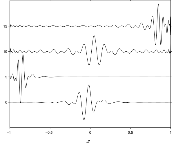
Figure 1: Wavelet functions \psi_{ji}(x) with scale index j = 5 and position indices i = 15, 5, 16, 26 from bottom to top. The lower two curves correspond to the present basis, while the upper two are the wavelets of Fröhlich and Uhlmann (2002).
